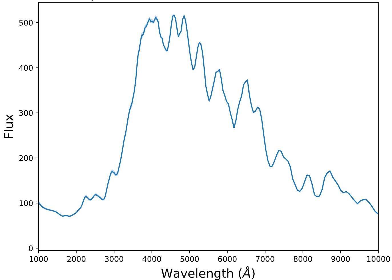
Spectrum 2 for transient CCSN at z=0.41
